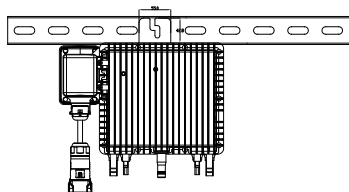
M6 / 80 / 100 G4 (2MPPT) Mounting
