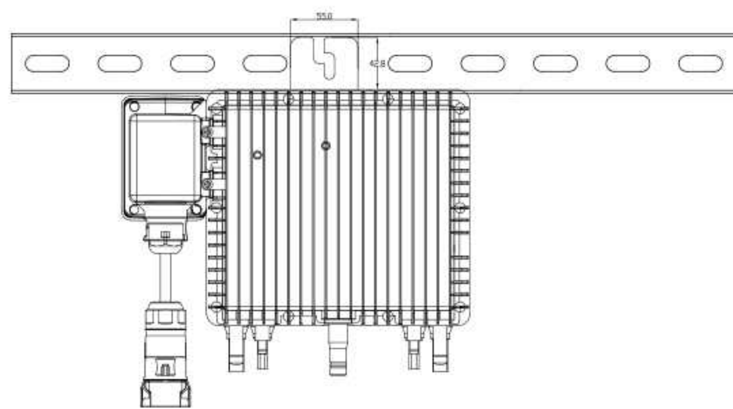
M60 / 80 / 100 G4 (2MPPT) Mounting
