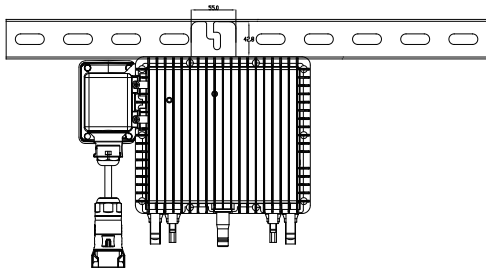
M60 / 80 / 100 G4 (2MPPT) Mounting
